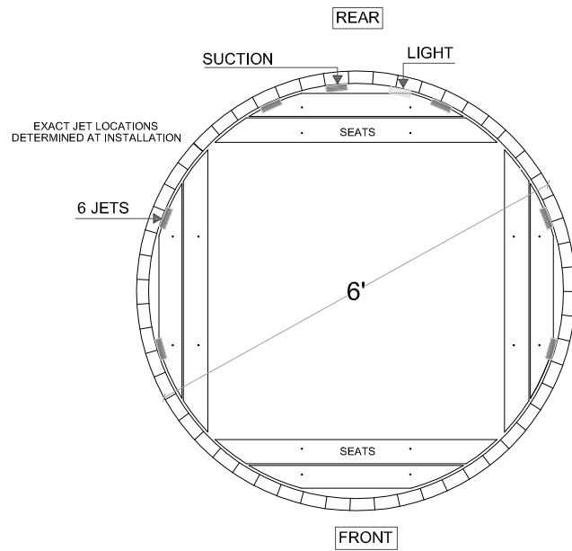
TOP PLAN
