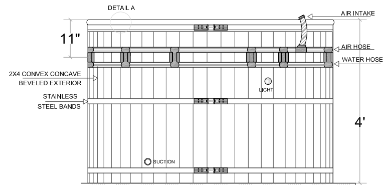
REAR ELEVATION
